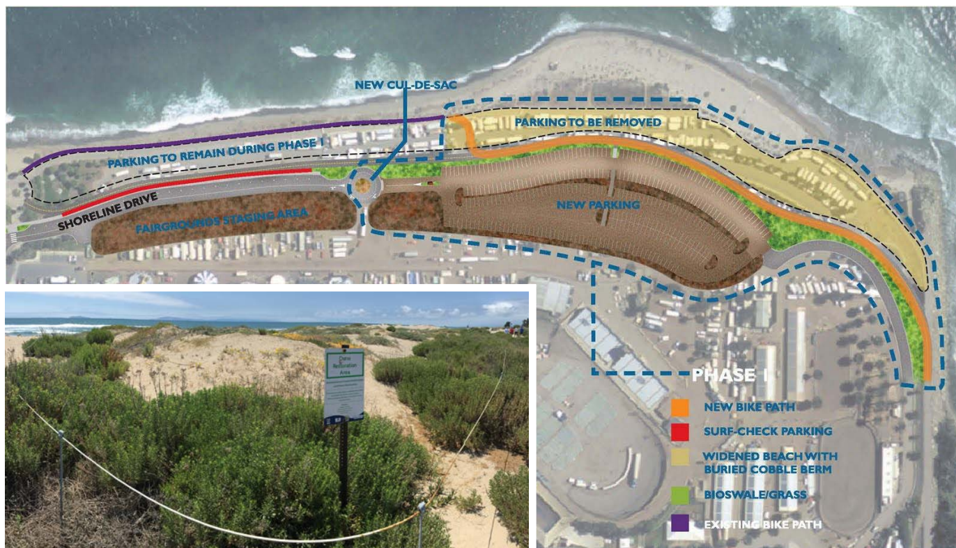
▲ Figure 11: A schematic showing the revised design to accommodate phasing due to budget constraints. Phase 1 (blue dashed lines) was constructed 2010-2012. The remainder of the project, called Phase 2 (highlighted shore areas to the left of Phase 1), has not been constructed. 2009. Image credit: City of Ventura, RRM and PWA. Inset Photo: Restored vegetated dunes in the area labeled as 'parking to be removed' in the design schematic. Photo credit: Paul Jenkin.
