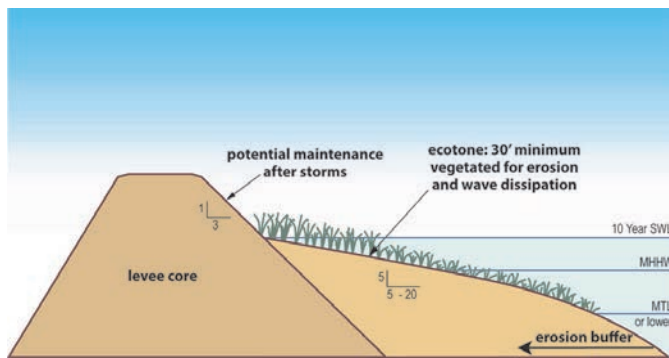
▲ Figure 27: Wave dampening bench showing levels at 10 Year Stillwater Level (SWL), Mean Higher High Water (MHHW) and Mean Tide Level (MTL). Image credit: ESA.
