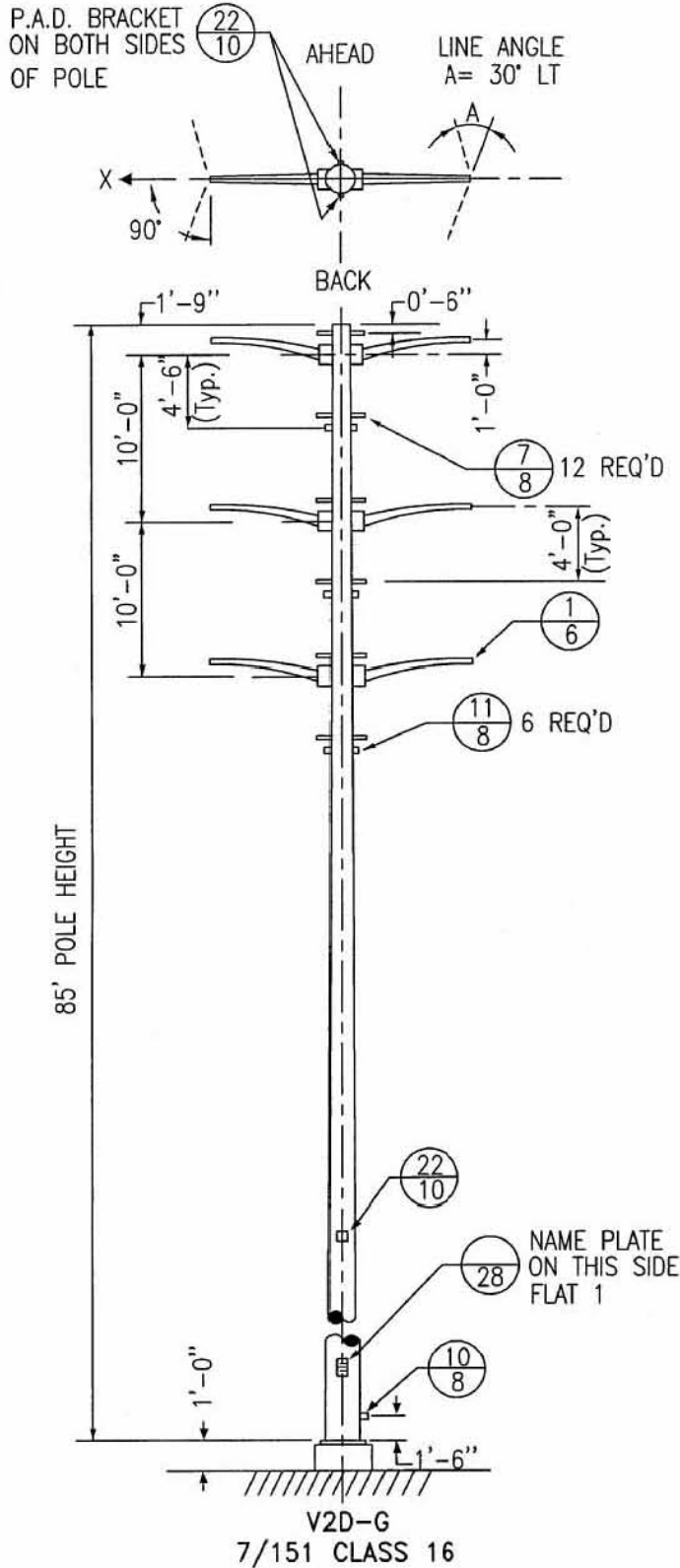
Tubular Steel Pole Example
