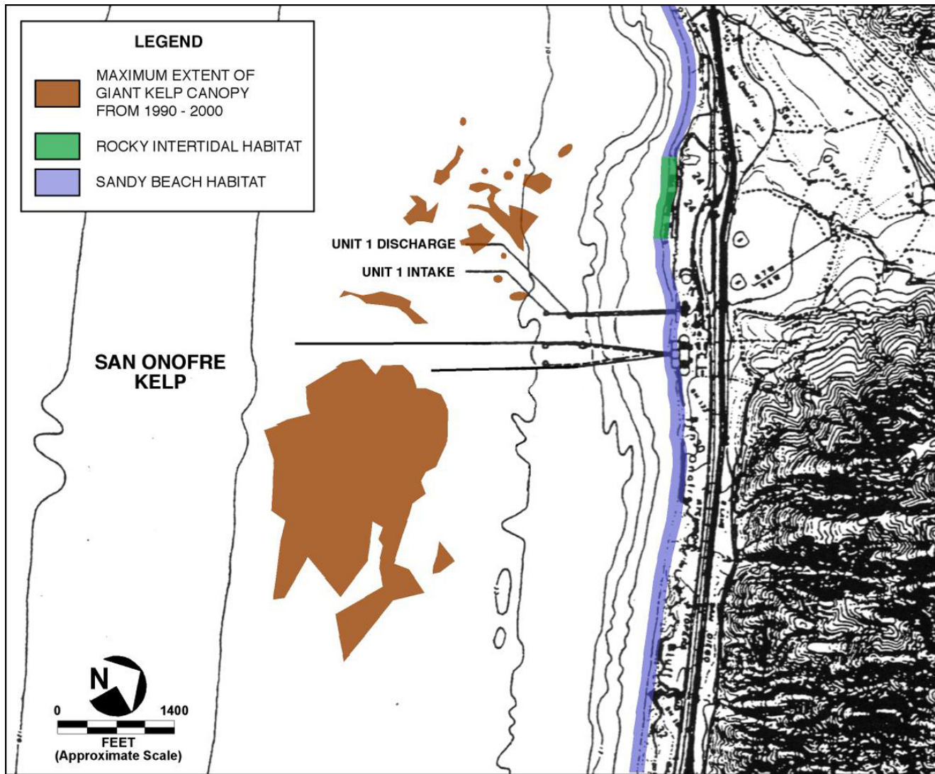
Figure 4.1-3 Distribution of Rocky and Sandy Intertidal Habitats and Extent of Giant Kelp Canopy
