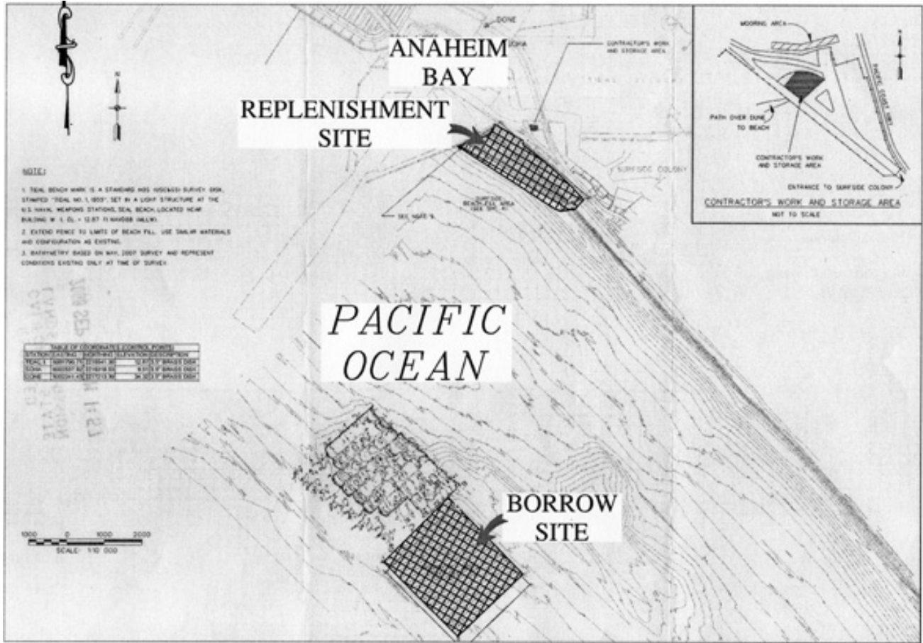
Stage 12 Dredging and Beach Replenishment Surfside-Sunset Beach
